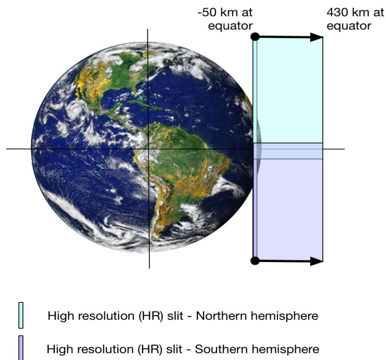
Figure 4-13 Limb Scan
