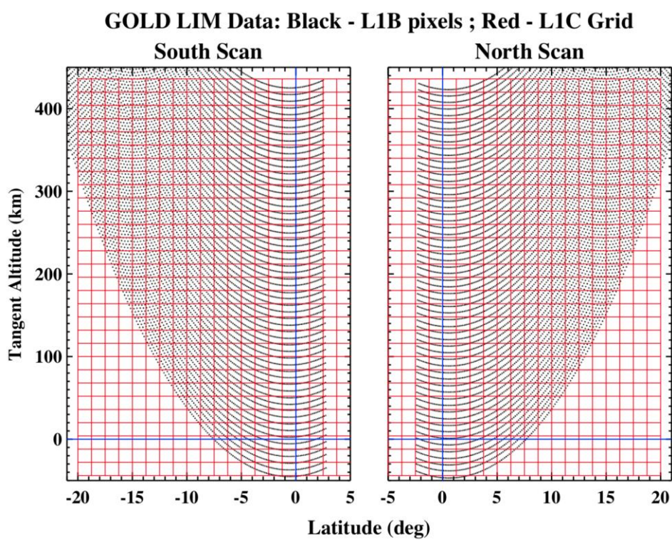
Figure 4-14 Grid for Limb Scan
