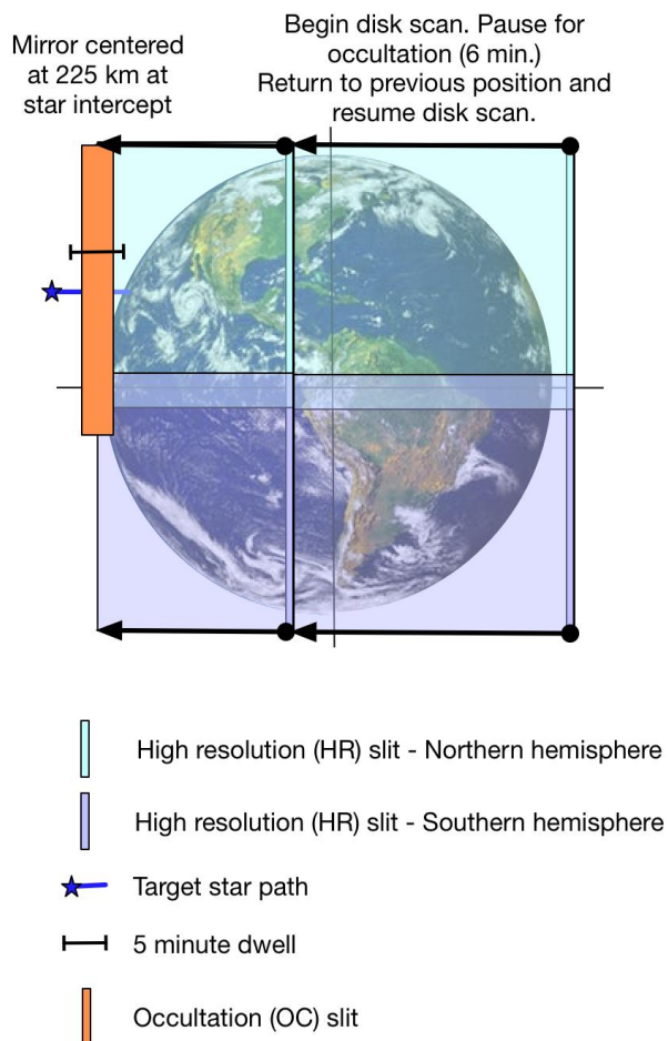
Figure 4-20 Occultation Observation
