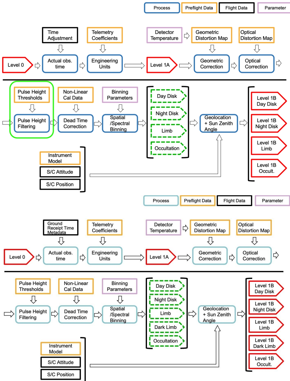
Figure 4-1 Level 0 to Level 1B Processing
