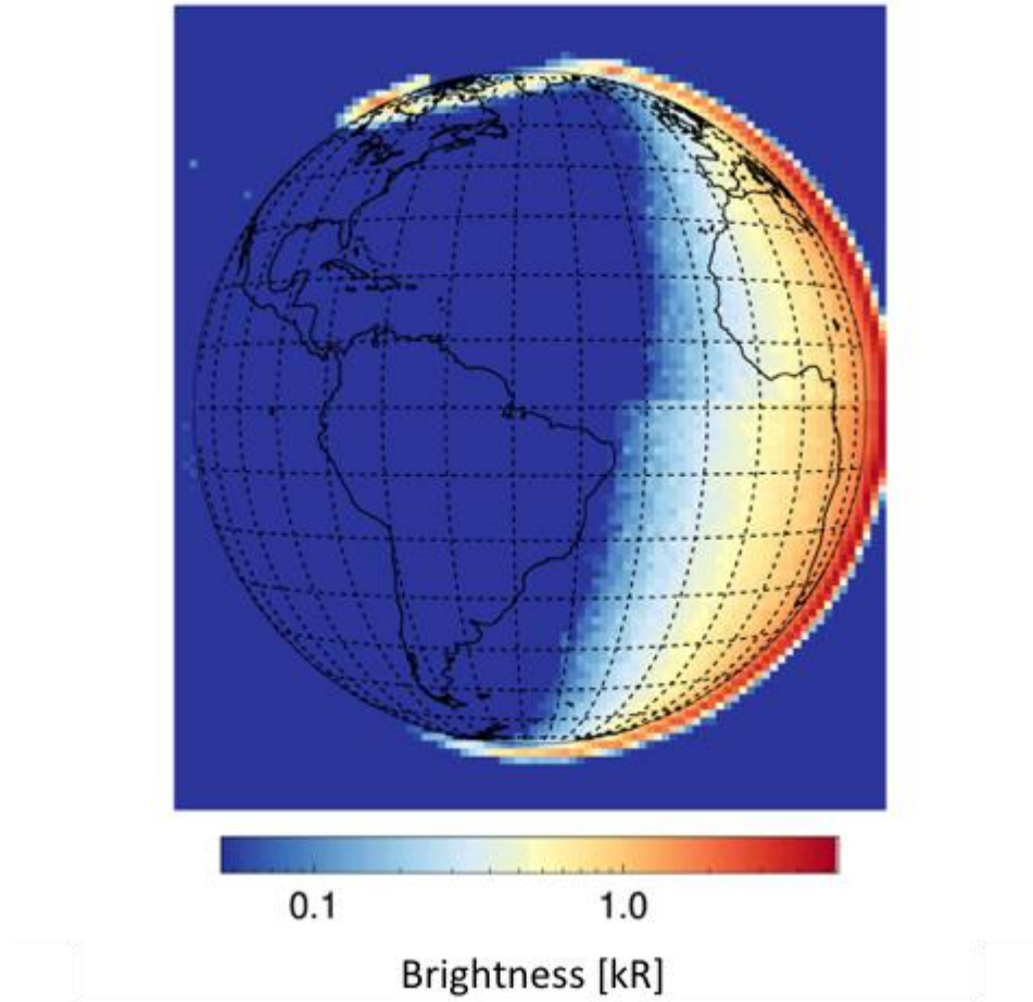
Figure 3-2 Combined scans of north and south latitudes from L1C data
