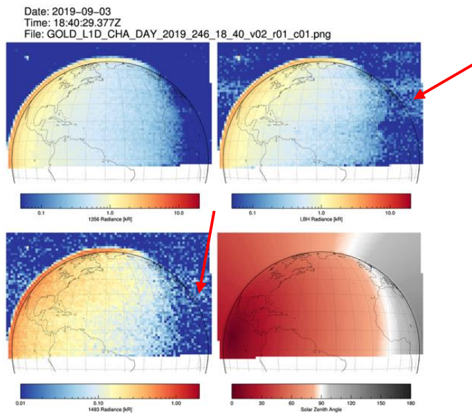
Figure 3-10 Noisy stripes in day time images; more prominent in the LBH emissions due to lower B(R) per pixel but higher background
