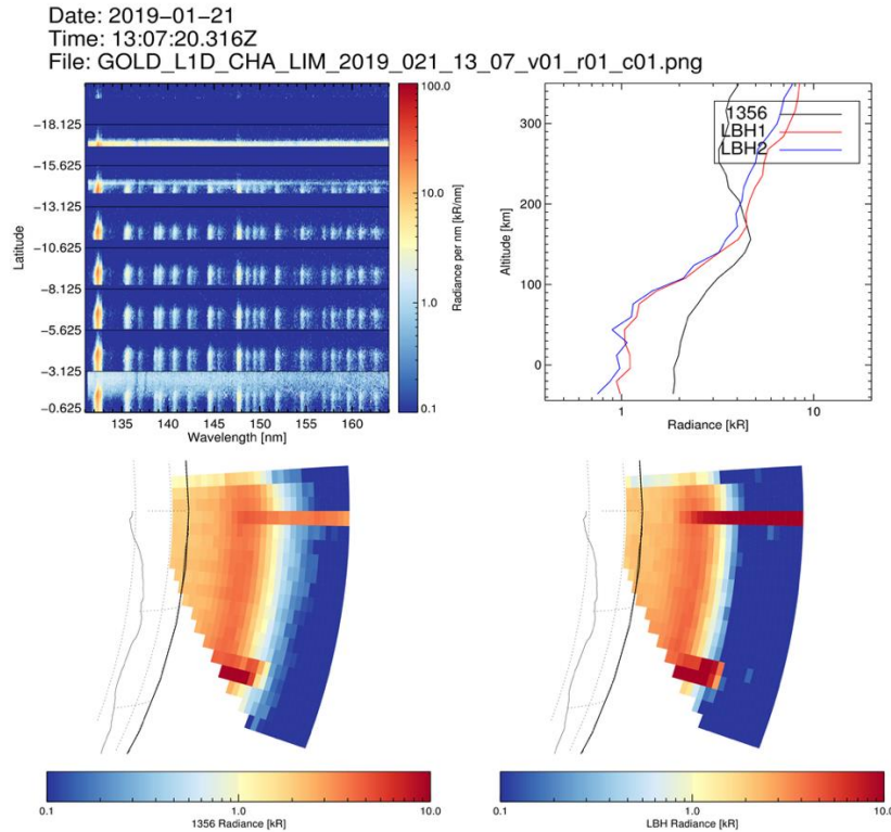
Figure 3-14 Level 1D plot showing observation of multiple stars in the field-of-view during a limb scan.
