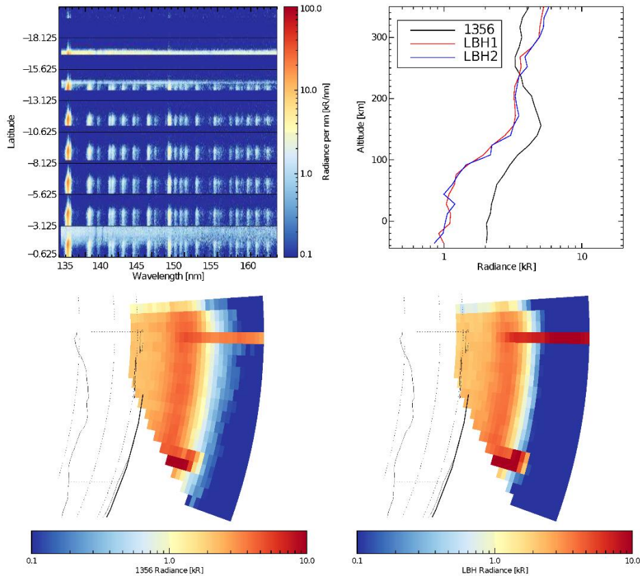
Figure 3-14 Level 1D plot showing observation of multiple stars in the field-of-view during a limb scan.
