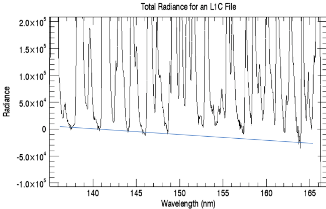
Figure 3-3 Wavelength Dependence Scattered Light
