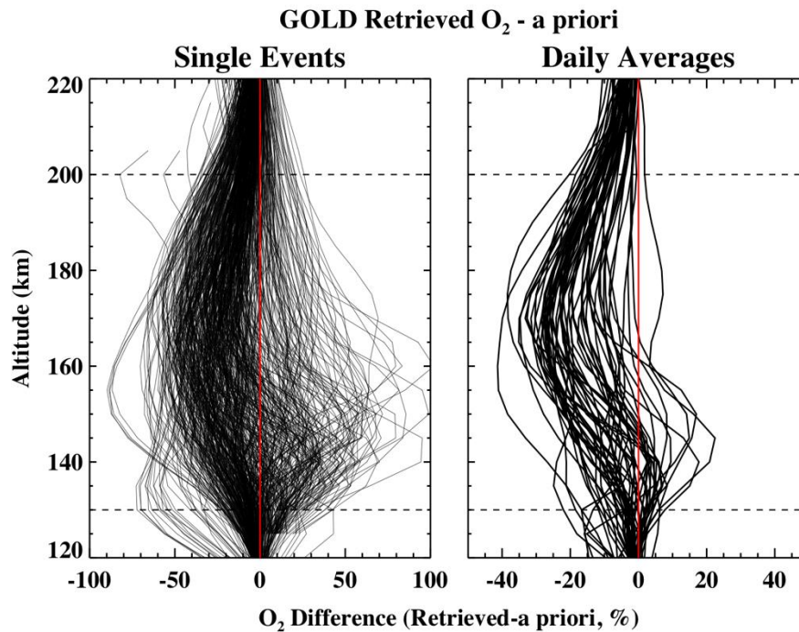
Figure 3-16 Variance between retrieved O 2 profile and retrieval a priori.
