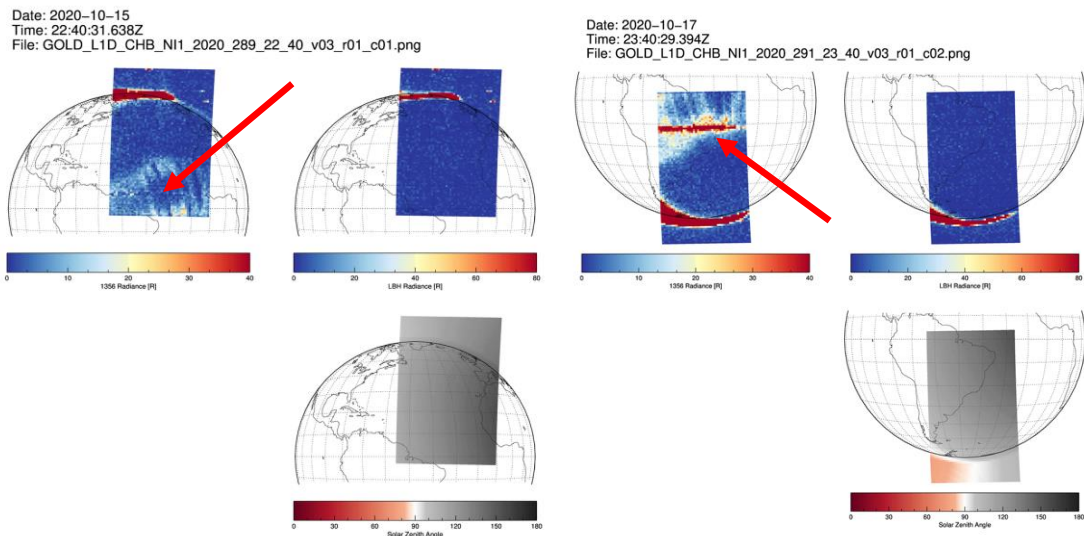
Figure 3-15 Horizontal stripes in Channel B NI1 scans due to limitations in the pulse height filtering and flat-field correction.
