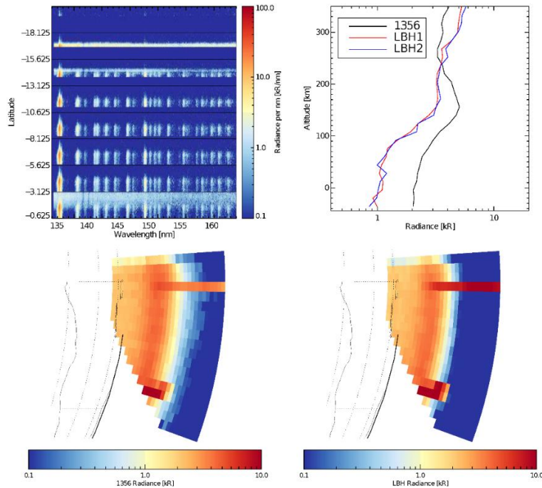
Figure 3-17 Level 1D plot showing observation of multiple stars in the field-of-view during a limb scan.
