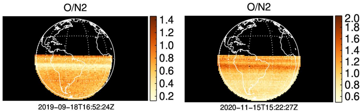
Figure 3-19 Examples of the impact of flat field correction errors on the ON2 data product. The errors result in horizontal bands of depleted or enhanced O/N 2
