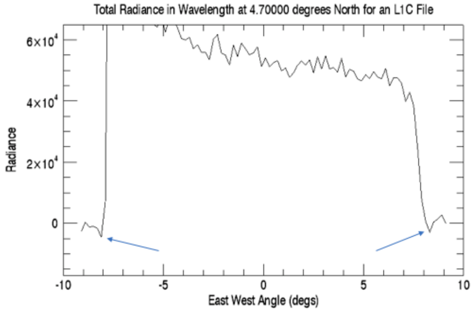
Figure 3-7 Over Corrected Background Subtraction at Limb
