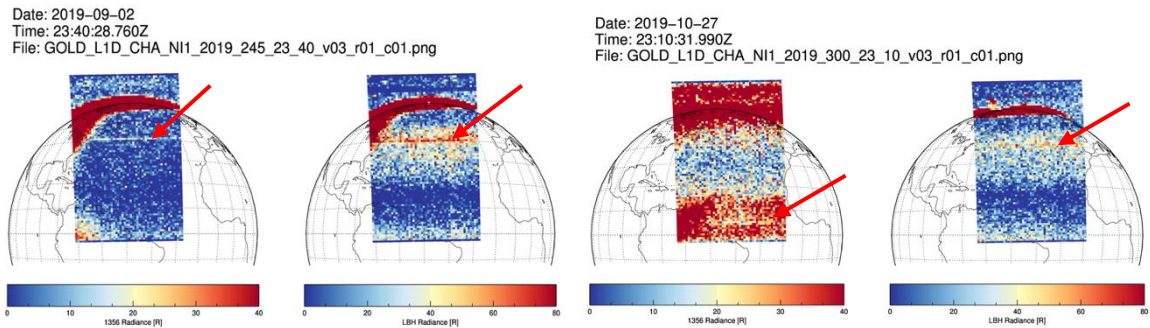
Figure 3-9 Examples of background noise appearing as horizontal stripes in night time images
