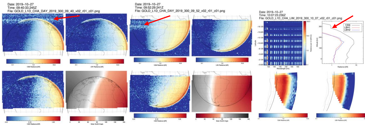
Figure 3-12 Horizontal stripes in observations with high particle background due to current limitations in the pulse height filtering, flat-field correction and background subtraction; more prominent in the OI 135.6 nm emission.
