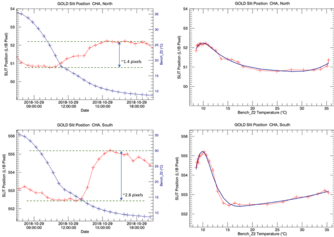
Figure 3-6 Vertical Slit Motion With Temperature
