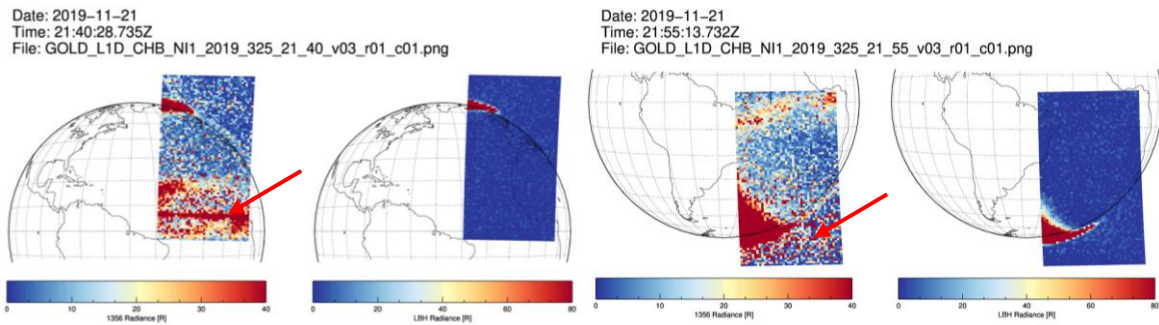
Figure 3-13 Horizontal stripes in Channel B night time scans due to incorrect current limitations in the pulse height filtering, flat-field correction and background subtraction; also seen in Channel A night time scans.
