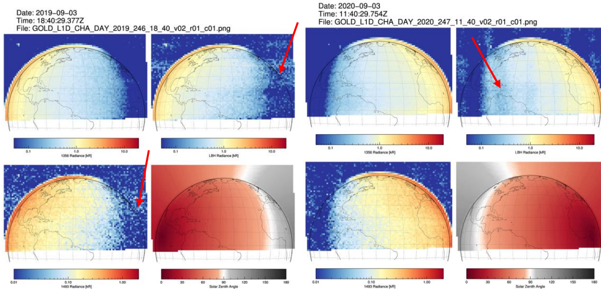
Figure 3-11 Noisy stripes in day time images; more prominent in the LBH emissions due to lower B(R) per pixel but higher background
