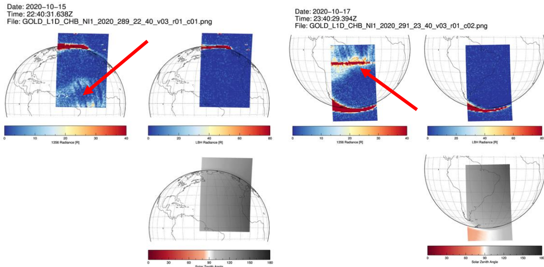
Figure 3-16 Horizontal stripes in Channel B NI1 scans due to limitations in the pulse height filtering and flat-field correction.
