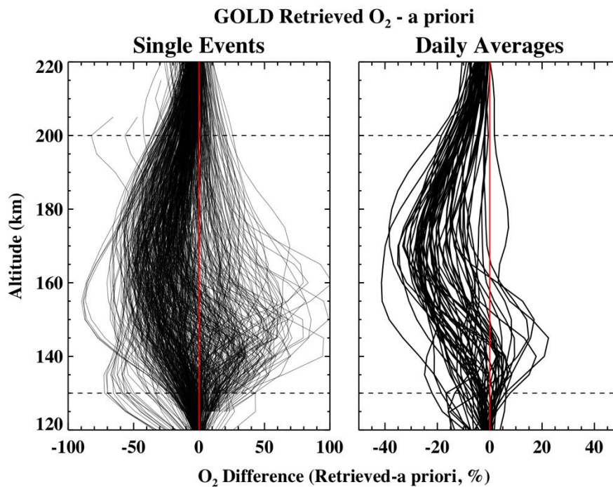
Figure 3-18 Variance between retrieved O 2 profile and retrieval a priori.
