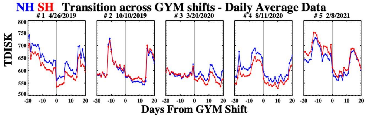
Figure 3-20 Daily average TDISK data before and after the five Channel A GYM shift operations to date. Northern/Southern hemisphere (NH/SH) are plotted in blue and red, respectively. In each panel the vertical solid line is the date of the GYM operation.
