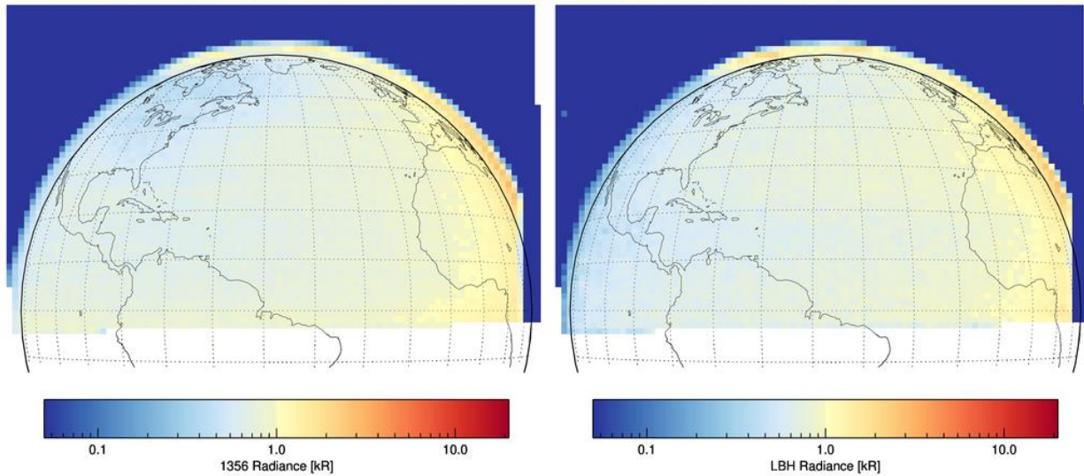
Figure 3-17 Artifact in DAY image after instrument safe-hold
