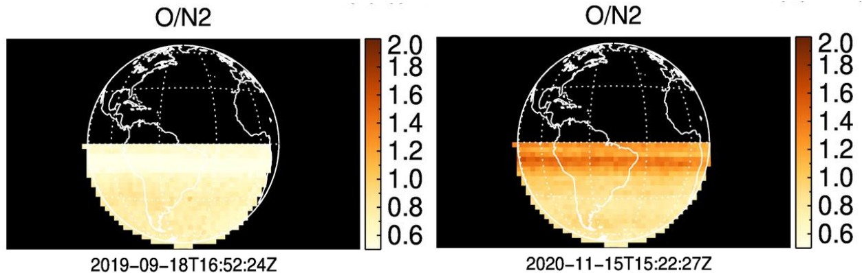
Figure 3-22 Examples of the impact of flat field correction errors on the ON2 data product. The errors result in horizontal bands of depleted or enhanced O/N 2
