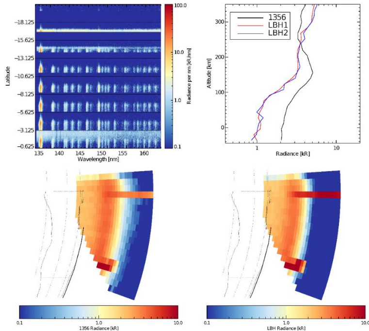
Figure 3-19 Level 1D plot showing observation of multiple stars in the field-of-view during a limb scan.
