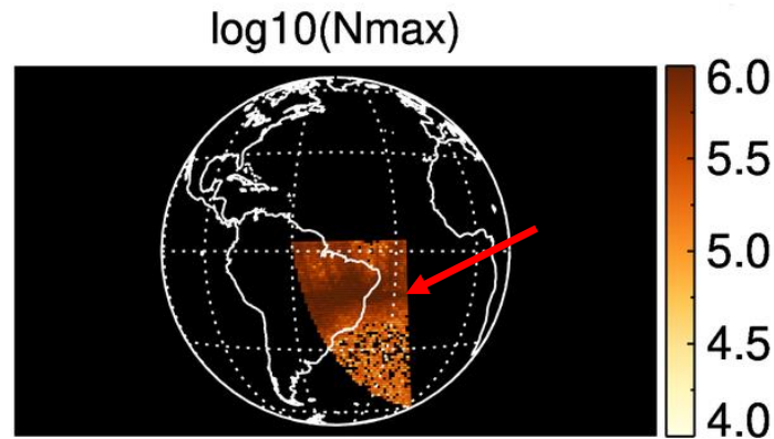
Figure 3-24 Horizontal stripe in the CHB NMAX data due to issues in the flat-field correction of the LIC NI1 data.
