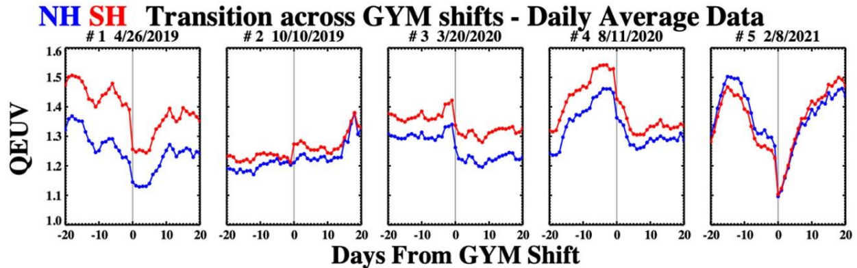
Figure 3-23 Daily average QEUV data before and after the five Channel A GYM shift operations to date. Northern/Southern hemisphere (NH/SH) are plotted in blue and red, respectively. In each panel the vertical solid line is the date of the GYM operation.
