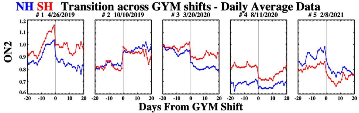
Figure 3-21 Daily average ON2 data before and after the five Channel A GYM shift operations to date. Northern/Southern hemisphere (NH/SH) are plotted in blue and red, respectively. In each panel the vertical solid line is the date of the GYM operation.
