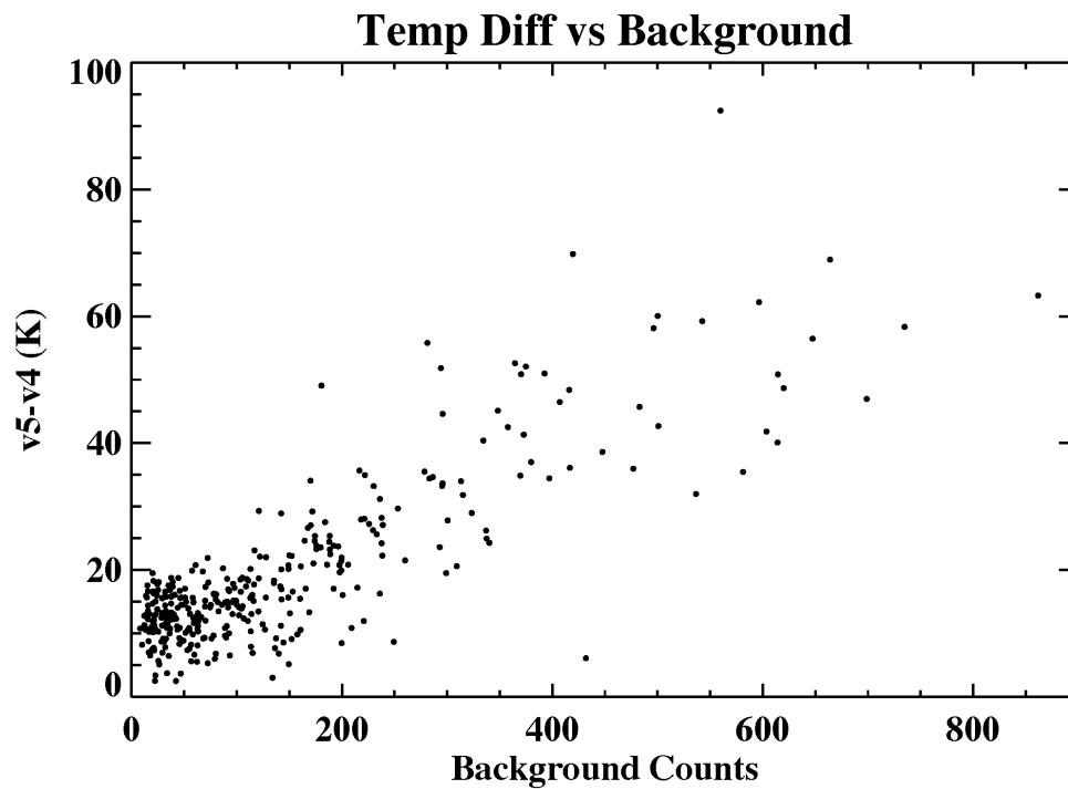
Figure 2-11 Scatterplot of \Delta\text{TLIMB} vs. background counts for the data shown in Figure 2-10
