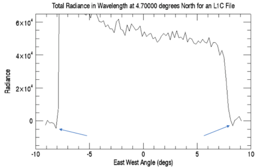
Figure 3-7 Over Corrected Background Subtraction at Limb
